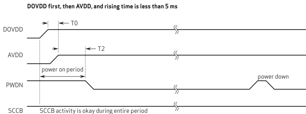
figure 2-2 power up timing with internal DVDD
