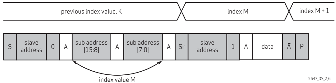
figure 2-5 SCCB single read from random location
