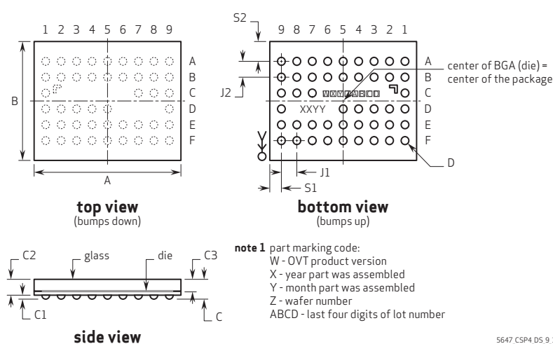
figure 9-1 package specifications
