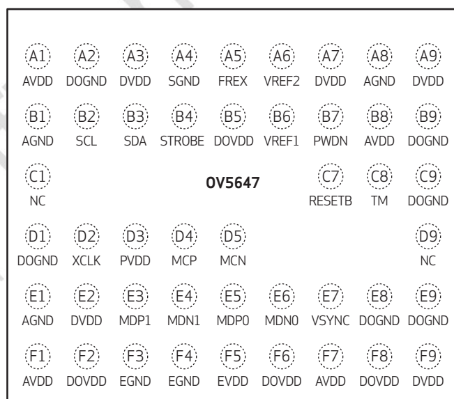
figure 1-1 pin diagram
