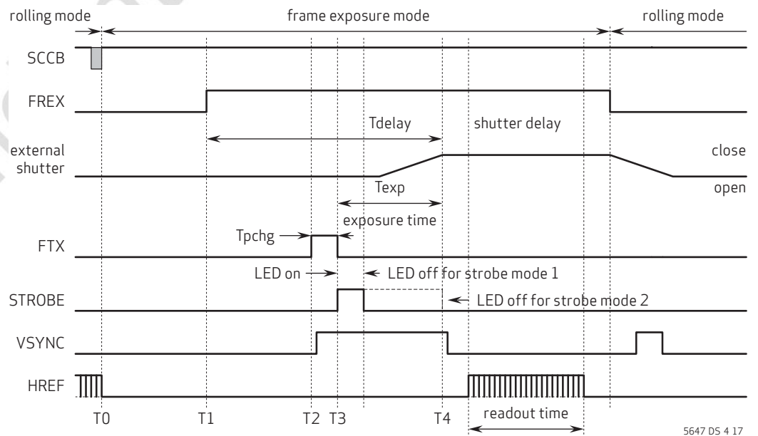
figure 4-17 STROBE control in FREX mode
