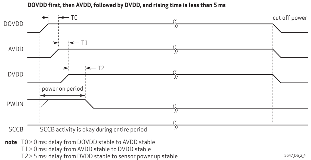
figure 2-3 power up timing with external DVDD source
