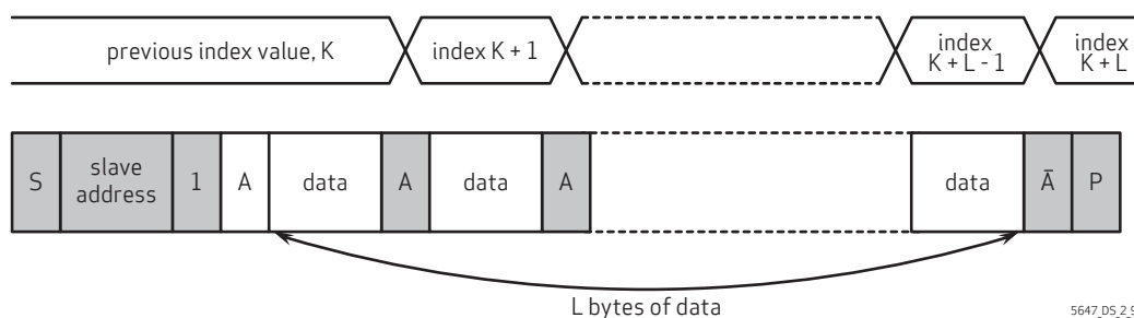
figure 2-8 SCCB sequential read from current location
